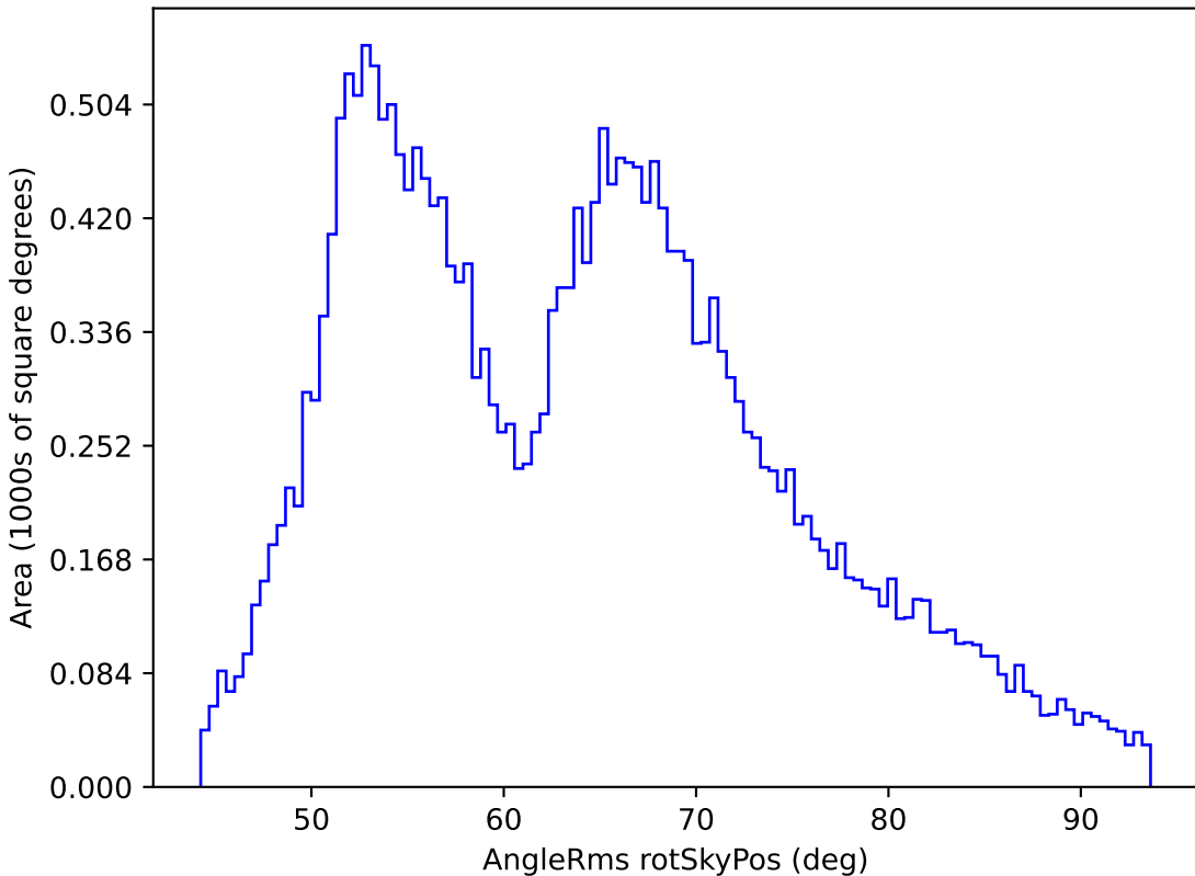
ddf_half_v3.4_10yrs All sky all bands: AngleRms rotSkyPos
