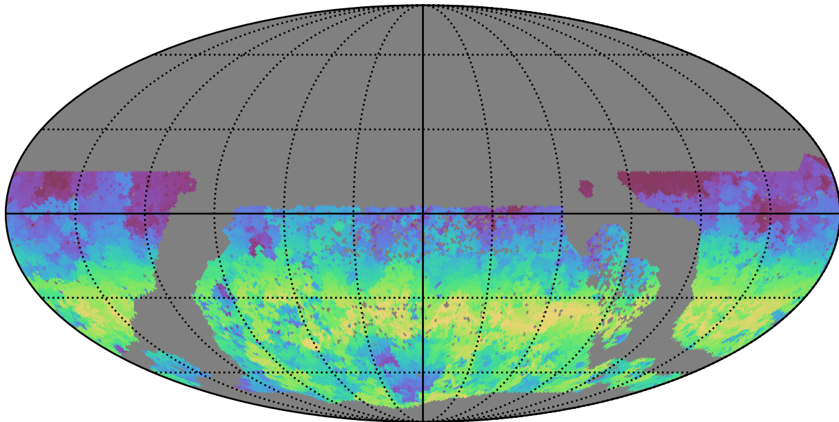
ddf_half_v3.4_10yrs WFD u band: AngleRange rotSkyPos
