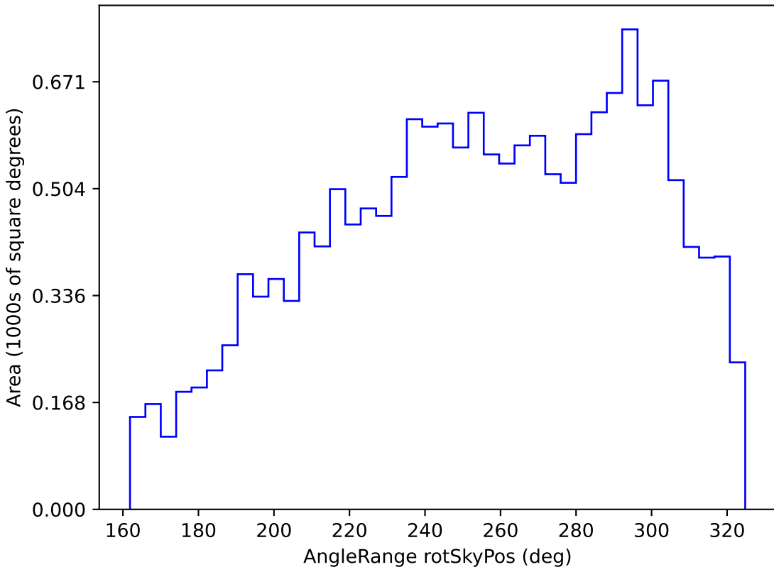
ddf_half_v3.4_10yrs WFD u band: AngleRange rotSkyPos
