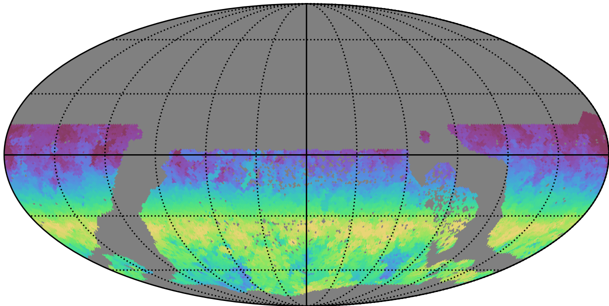
ddf_half_v3.4_10yrs WFD r band: AngleRange rotSkyPos
