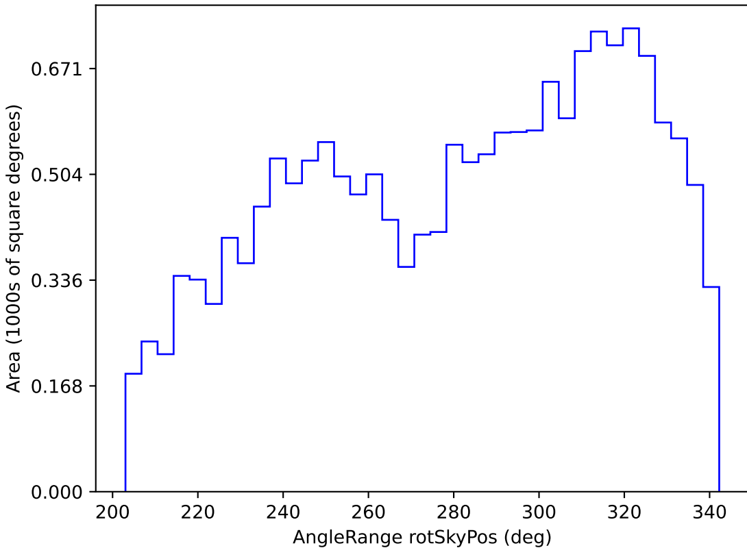
ddf_half_v3.4_10yrs WFD i band: AngleRange rotSkyPos
