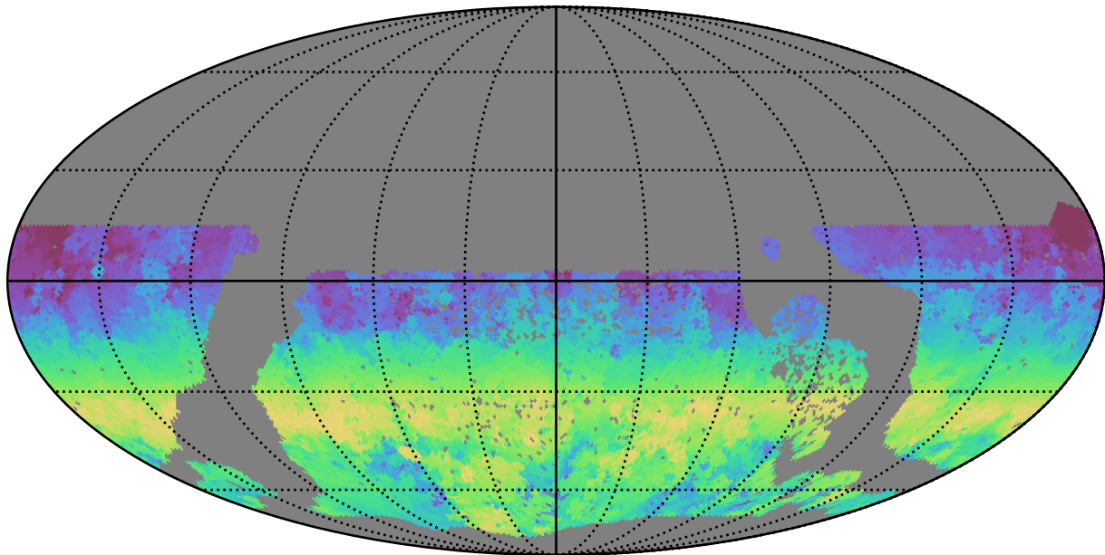
ddf_half_v3.4_10yrs WFD g band: AngleRange rotSkyPos
