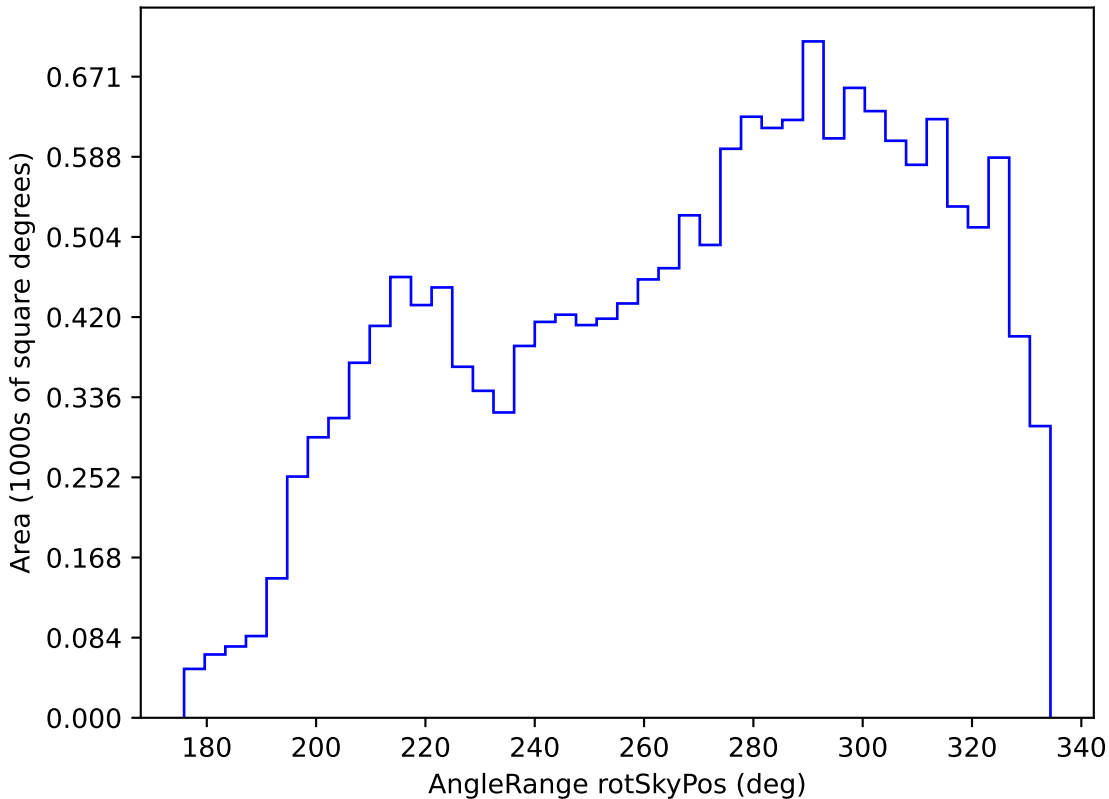
ddf_half_v3.4_10yrs WFD g band: AngleRange rotSkyPos
