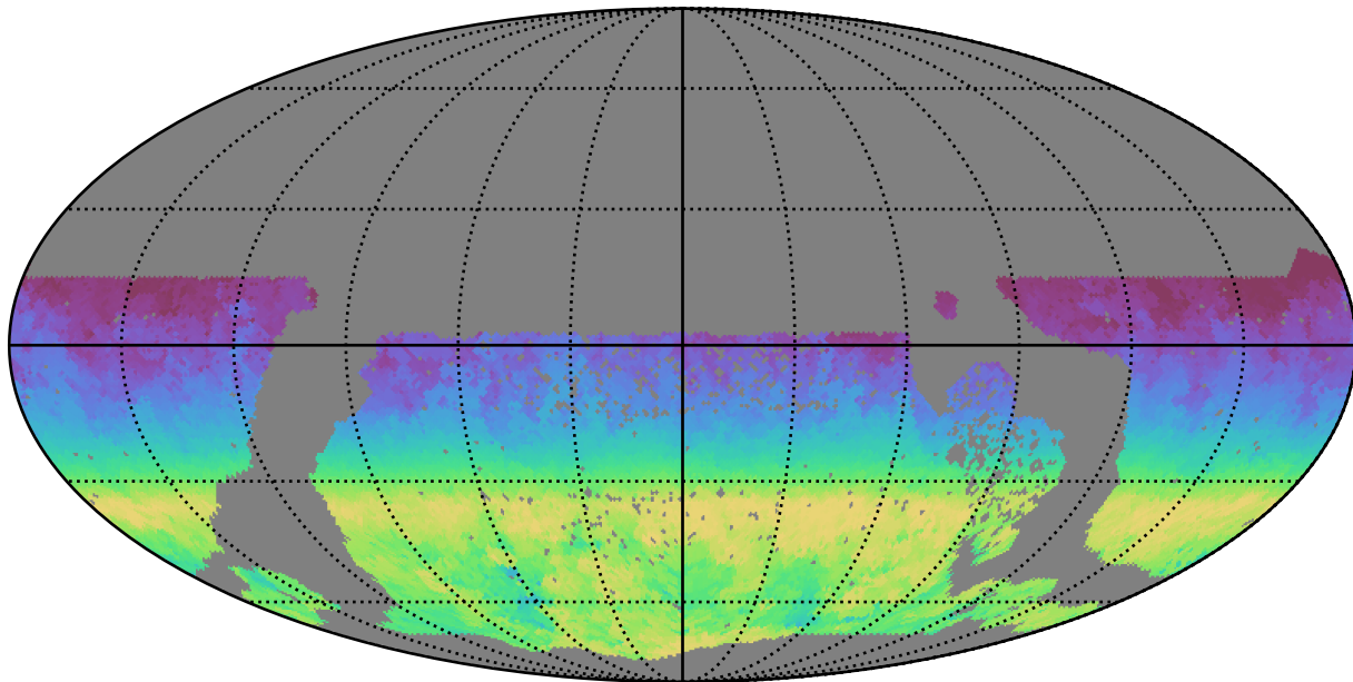
ddf_half_v3.4_10yrs WFD all bands: AngleRange rotSkyPos
