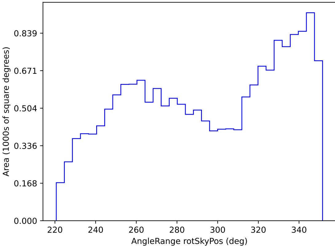
ddf_half_v3.4_10yrs WFD all bands: AngleRange rotSkyPos
