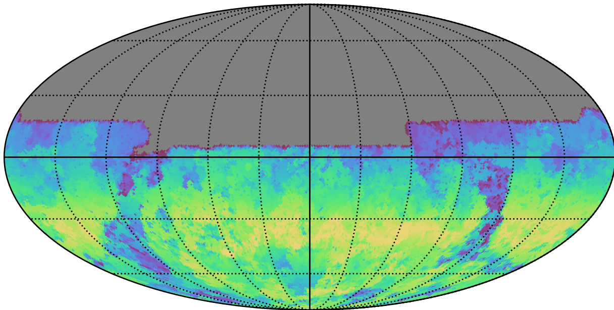
ddf_half_v3.4_10yrs All sky u band: AngleRange rotSkyPos
