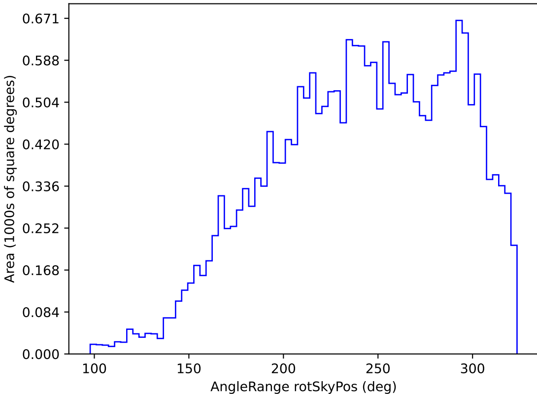
ddf_half_v3.4_10yrs All sky u band: AngleRange rotSkyPos
