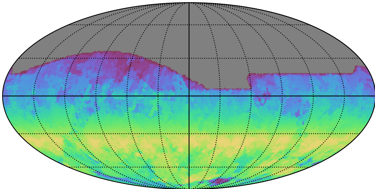
ddf_half_v3.4_10yrs All sky r band: AngleRange rotSkyPos
