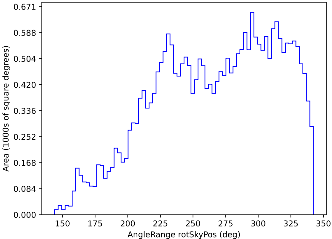
ddf_half_v3.4_10yrs All sky r band: AngleRange rotSkyPos
