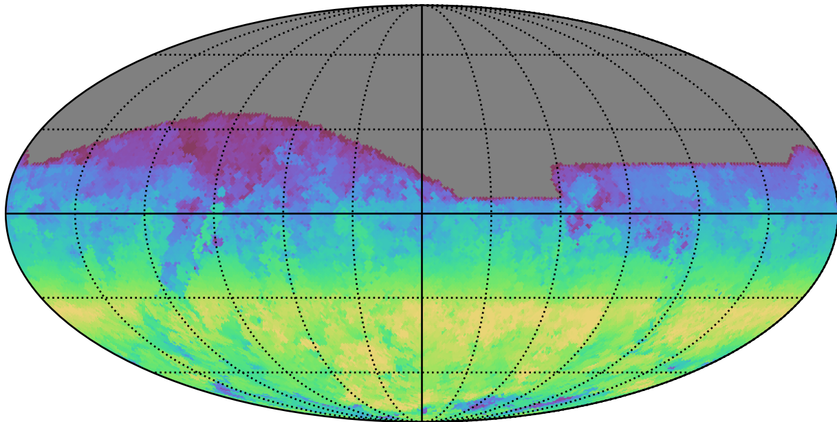
ddf_half_v3.4_10yrs All sky i band: AngleRange rotSkyPos
