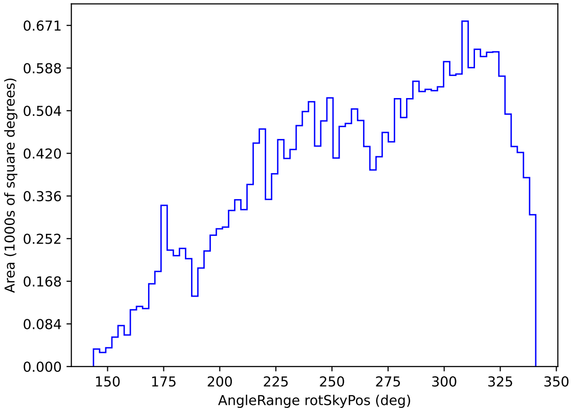
ddf_half_v3.4_10yrs All sky i band: AngleRange rotSkyPos
