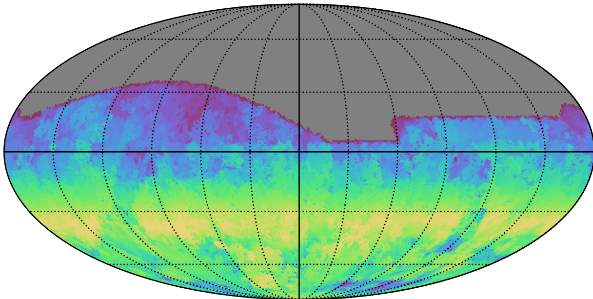
ddf_half_v3.4_10yrs All sky g band: AngleRange rotSkyPos
