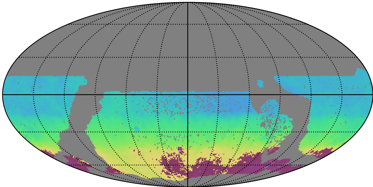
ddf_half_v3.4_10yrs WFD z band: AngleMean rotSkyPos
