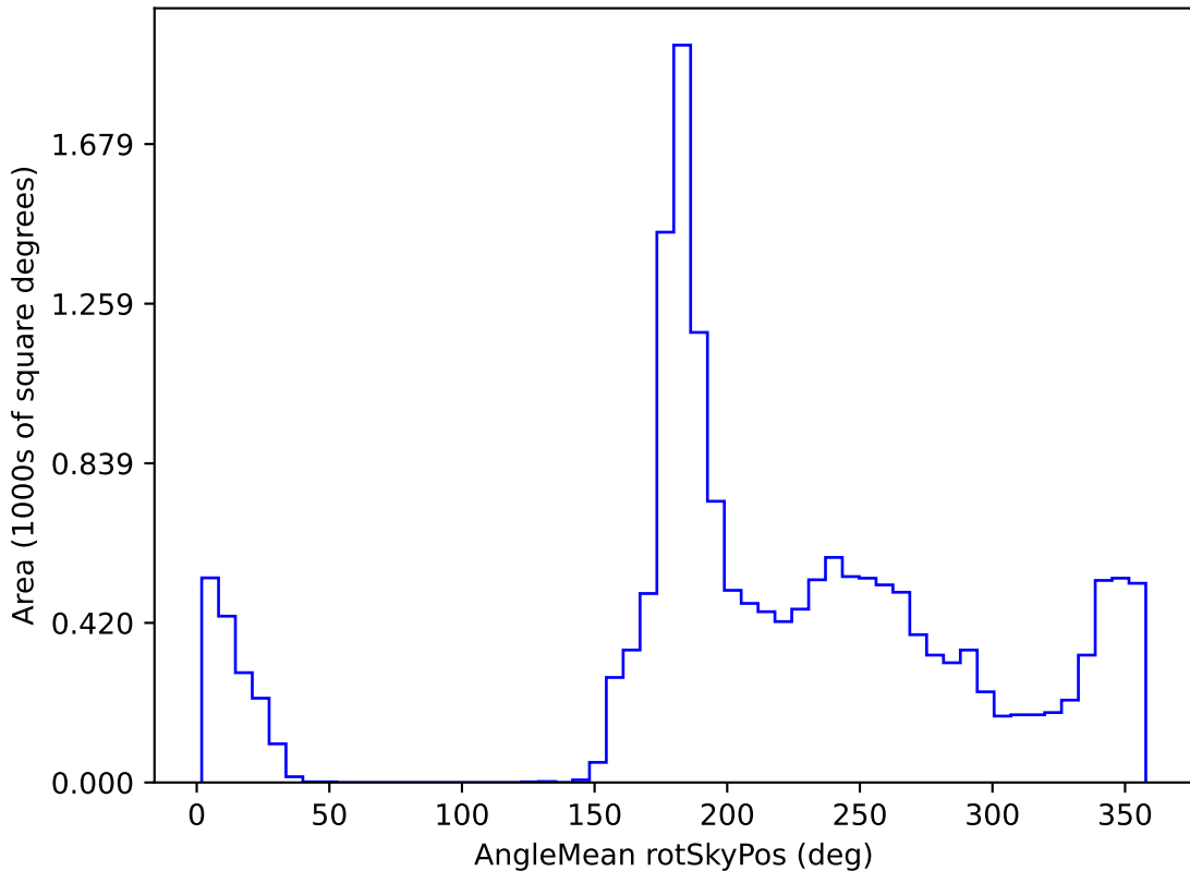
ddf_half_v3.4_10yrs WFD z band: AngleMean rotSkyPos
