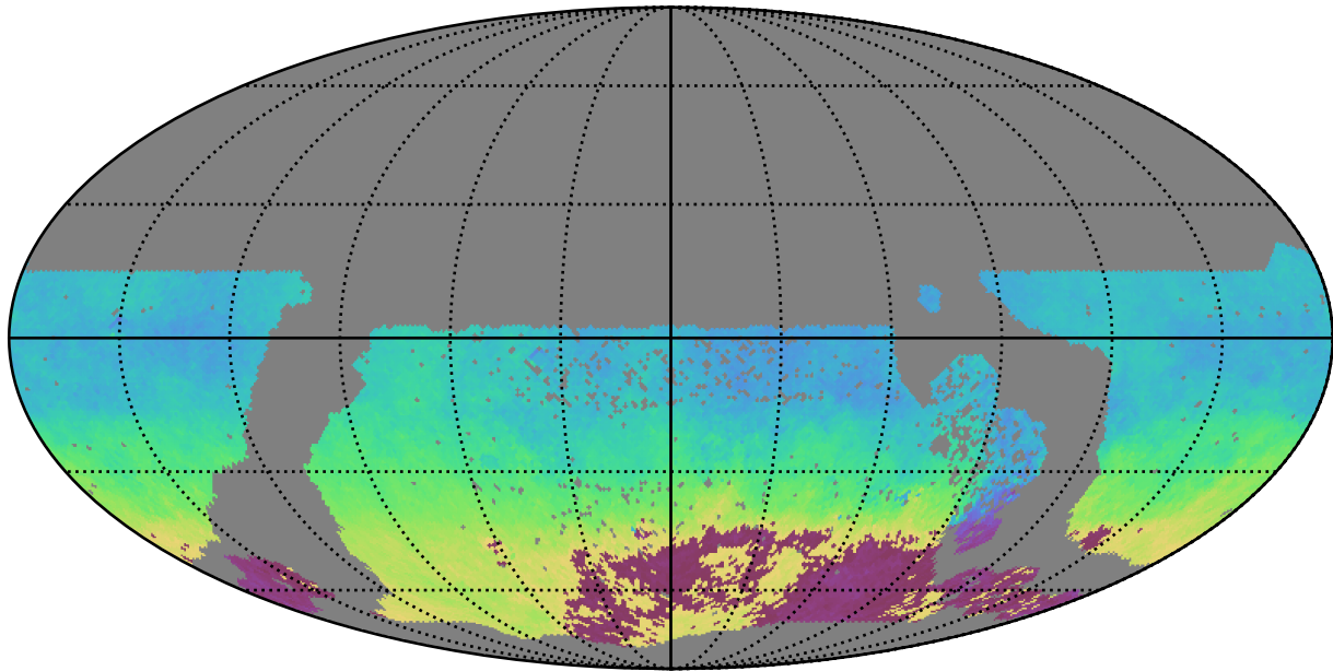
ddf_half_v3.4_10yrs WFD u band: AngleMean rotSkyPos
