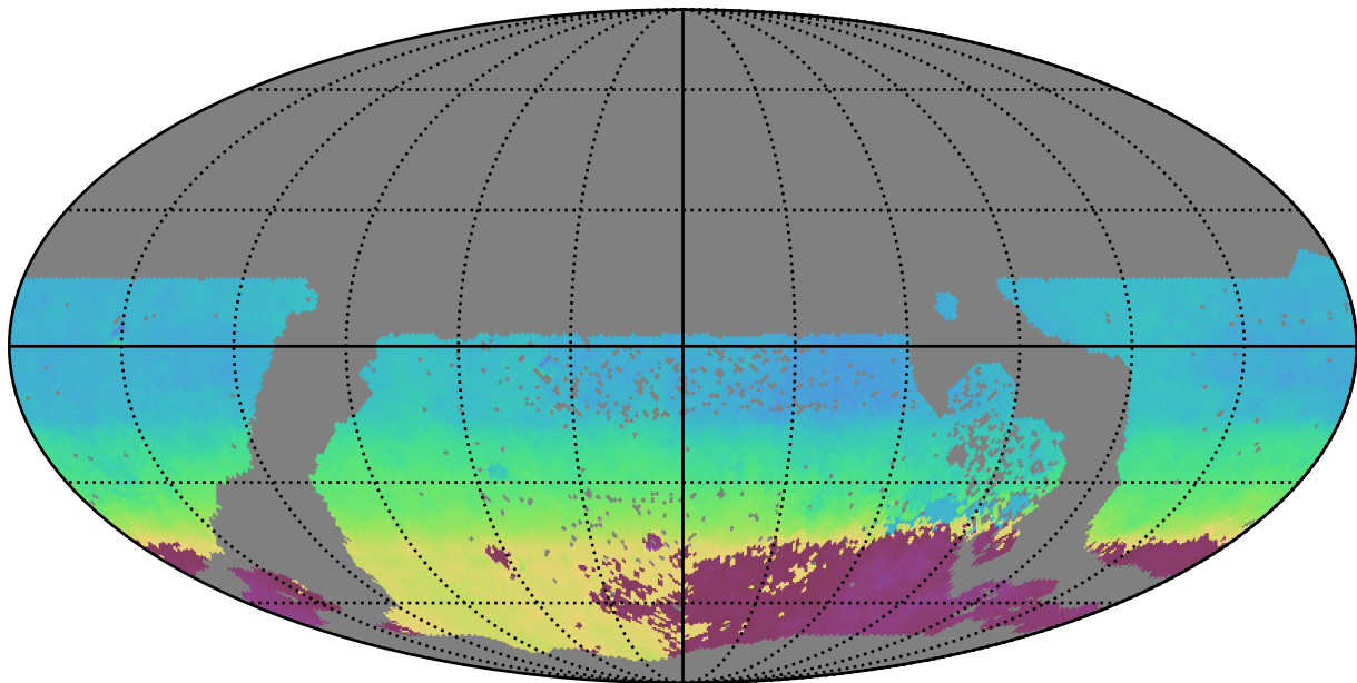
ddf_half_v3.4_10yrs WFD r band: AngleMean rotSkyPos
