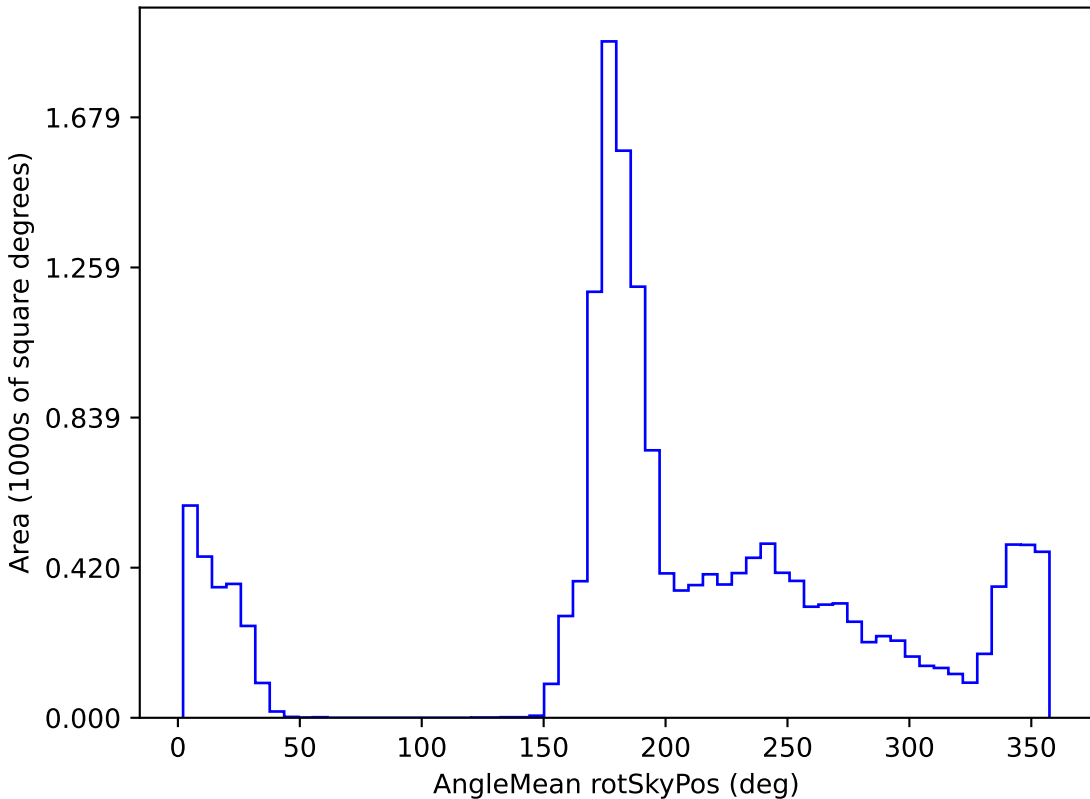
ddf_half_v3.4_10yrs WFD r band: AngleMean rotSkyPos
