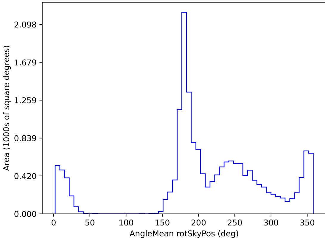
ddf_half_v3.4_10yrs WFD i band: AngleMean rotSkyPos
