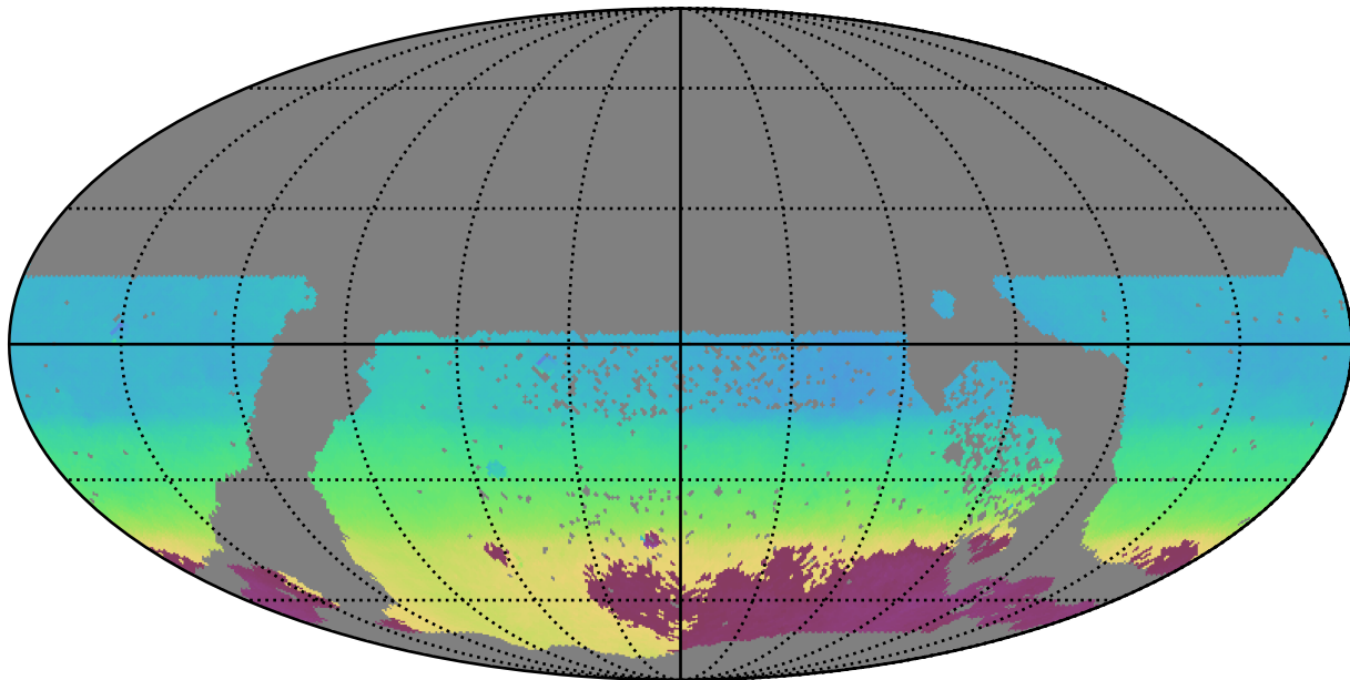
ddf_half_v3.4_10yrs WFD all bands: AngleMean rotSkyPos
