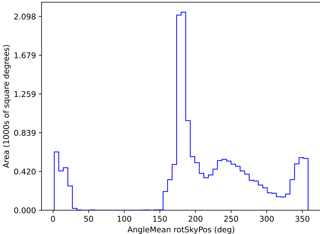
ddf_half_v3.4_10yrs WFD all bands: AngleMean rotSkyPos
