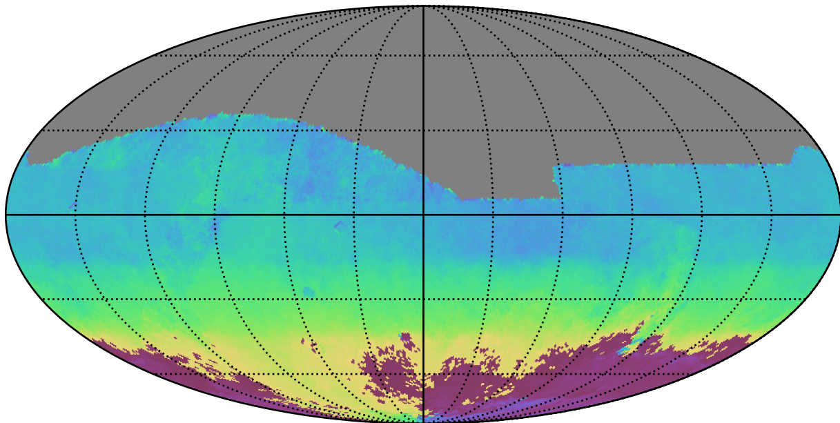
ddf_half_v3.4_10yrs All sky z band: AngleMean rotSkyPos
