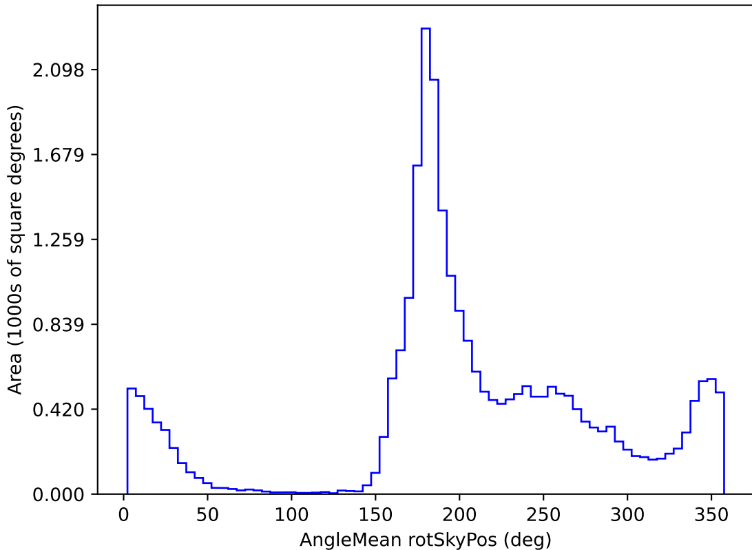
ddf_half_v3.4_10yrs All sky z band: AngleMean rotSkyPos
