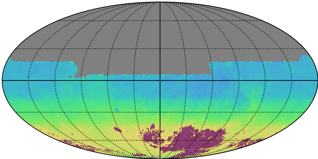
ddf_half_v3.4_10yrs All sky y band: AngleMean rotSkyPos
