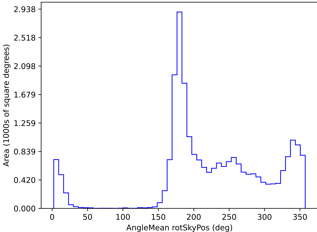
ddf_half_v3.4_10yrs All sky y band: AngleMean rotSkyPos
