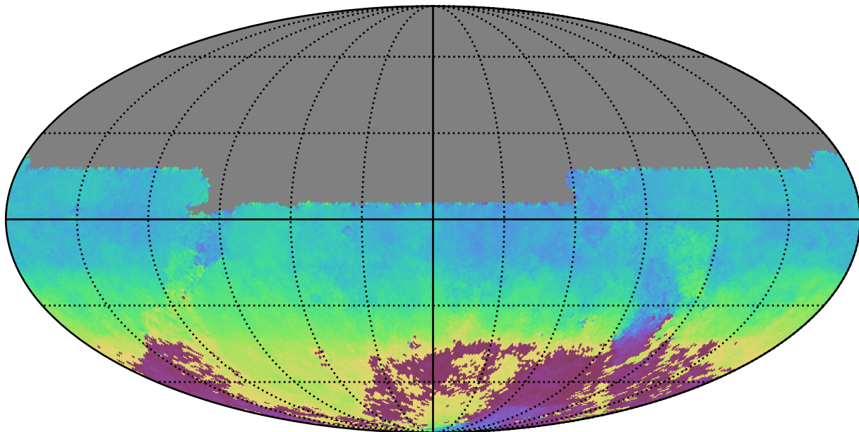
ddf_half_v3.4_10yrs All sky u band: AngleMean rotSkyPos
