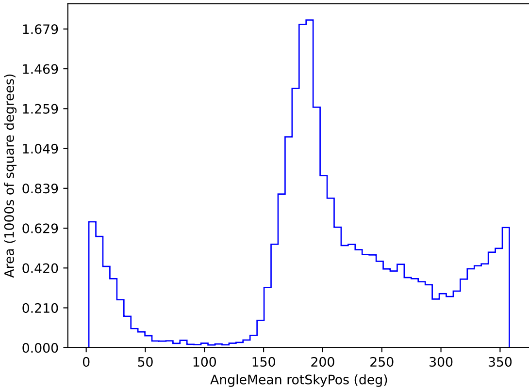
ddf_half_v3.4_10yrs All sky u band: AngleMean rotSkyPos
