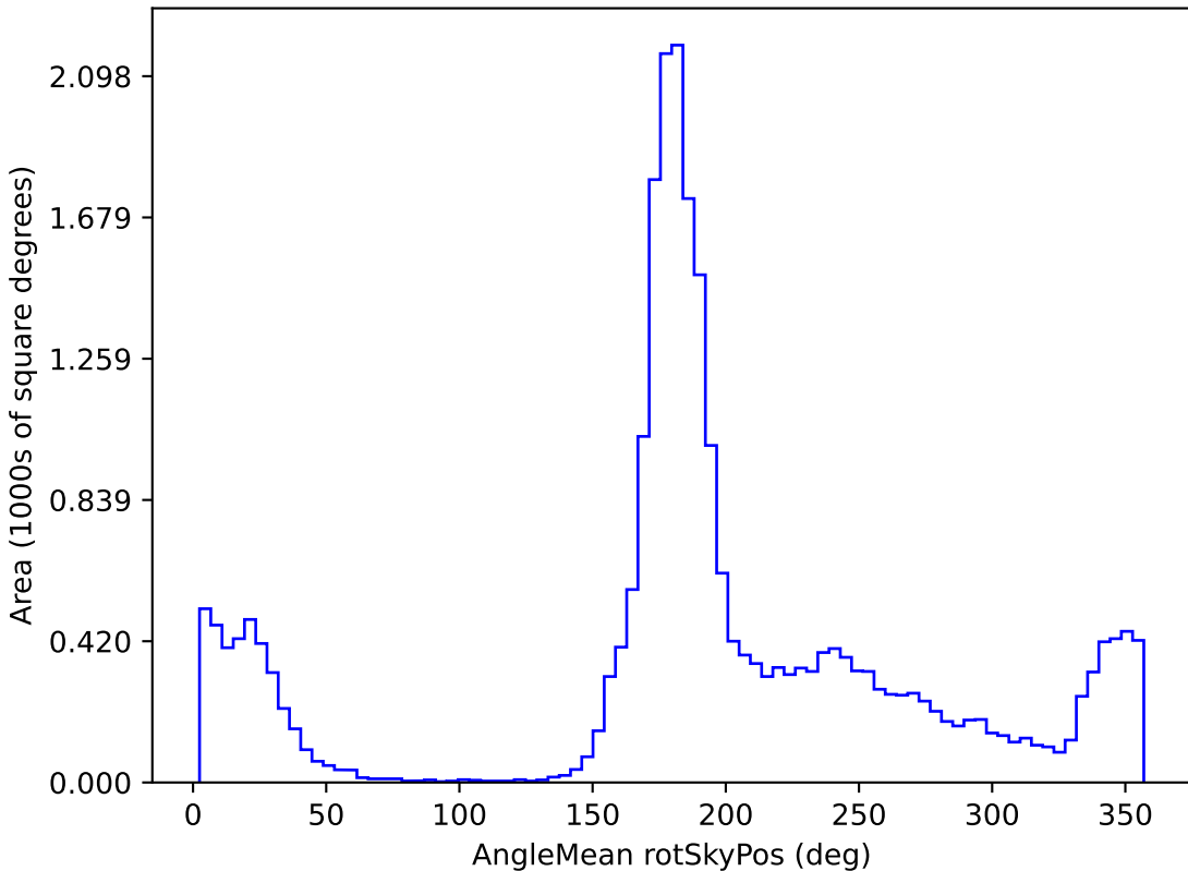
ddf_half_v3.4_10yrs All sky r band: AngleMean rotSkyPos
