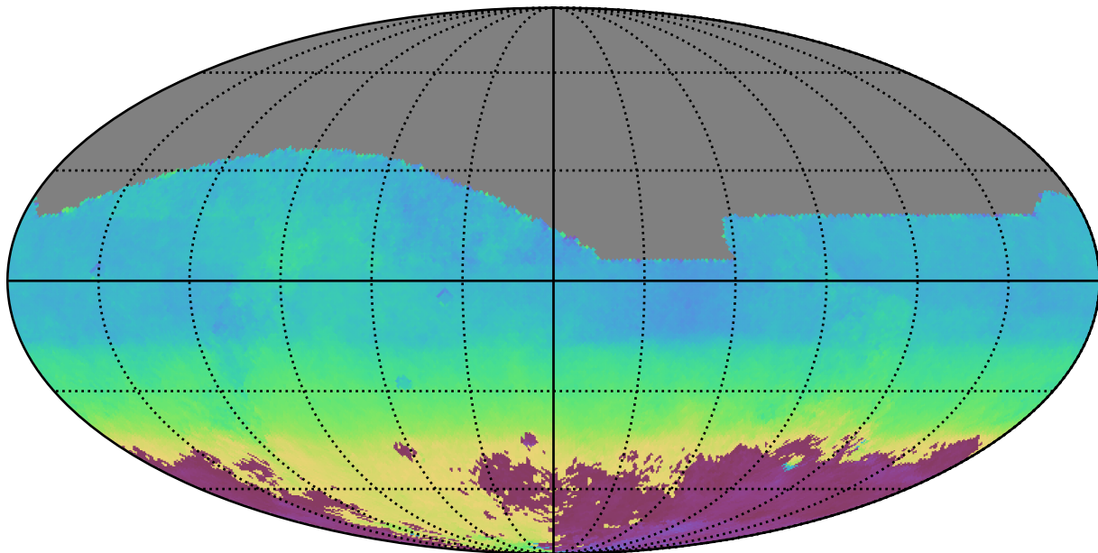
ddf_half_v3.4_10yrs All sky i band: AngleMean rotSkyPos
