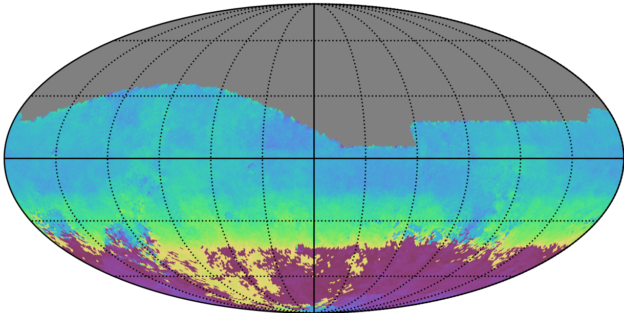
ddf_half_v3.4_10yrs All sky g band: AngleMean rotSkyPos
