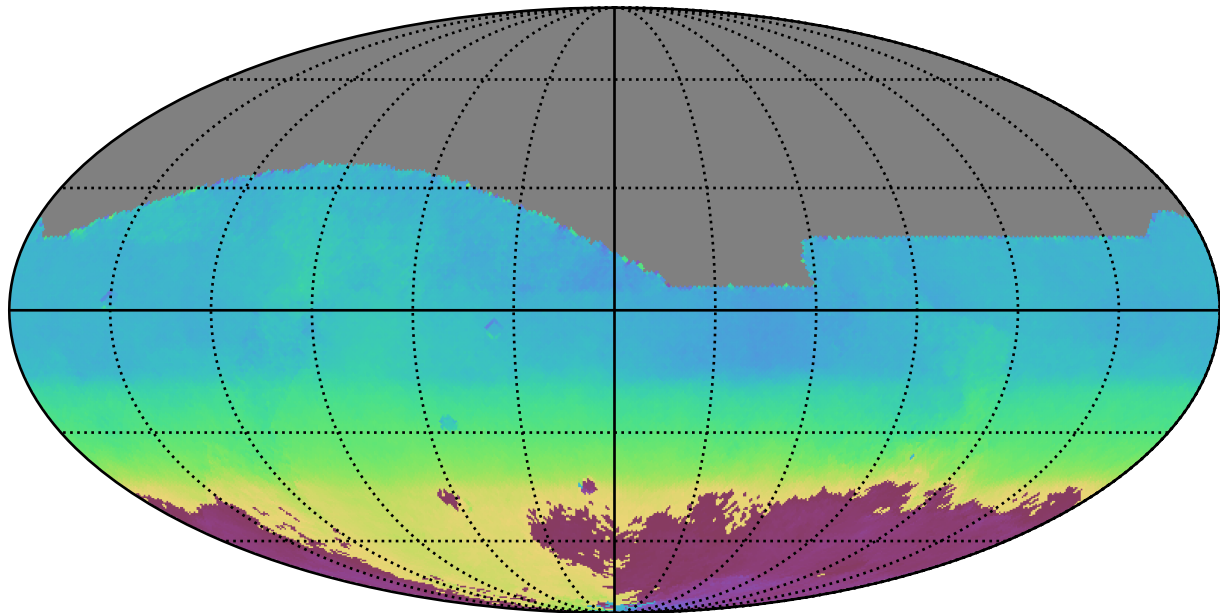
ddf_half_v3.4_10yrs All sky all bands: AngleMean rotSkyPos
