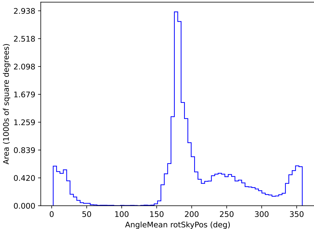
ddf_half_v3.4_10yrs All sky all bands: AngleMean rotSkyPos
