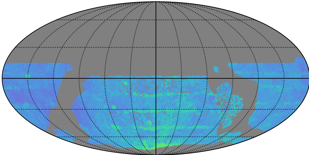
ddf_half_v3.4_10yrs WFD z band: 80thPercentile Season Length
