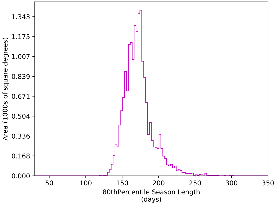
ddf_half_v3.4_10yrs WFD z band: 80thPercentile Season Length
