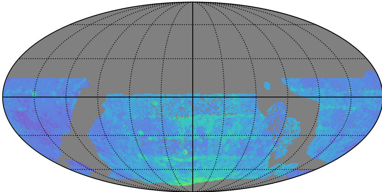
ddf_half_v3.4_10yrs WFD y band: 80thPercentile Season Length
