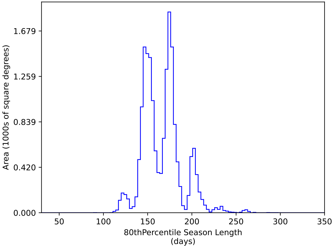
ddf_half_v3.4_10yrs WFD y band: 80thPercentile Season Length
