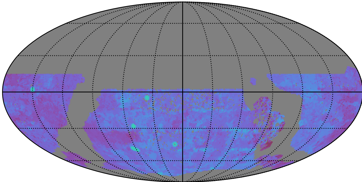
ddf_half_v3.4_10yrs WFD u band: 80thPercentile Season Length
