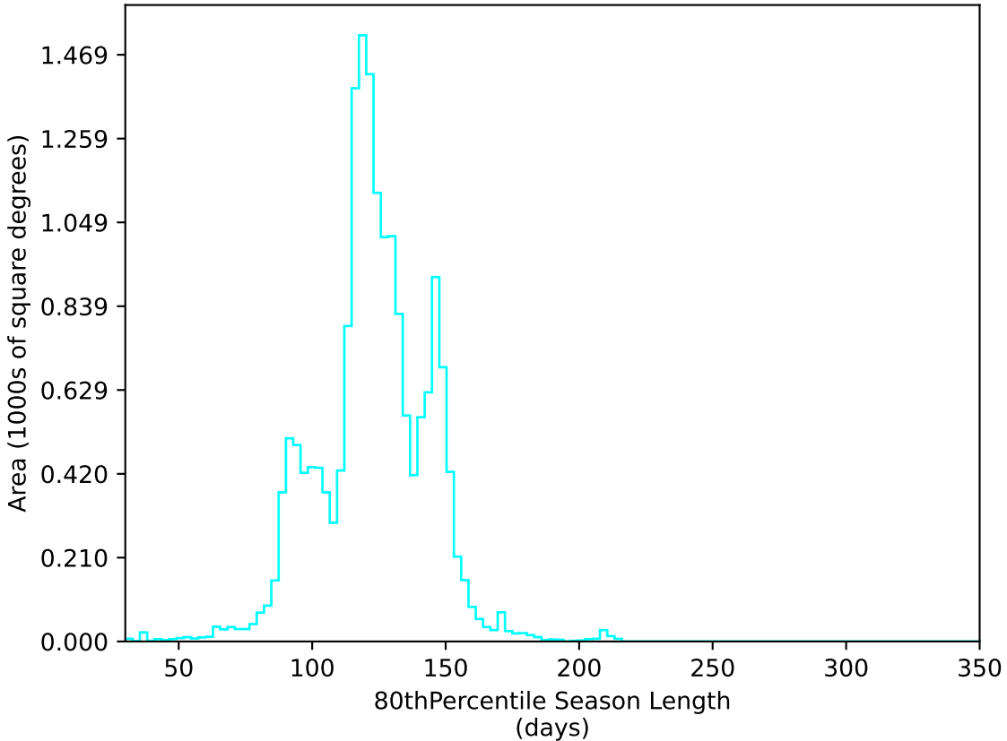
ddf_half_v3.4_10yrs WFD u band: 80thPercentile Season Length
