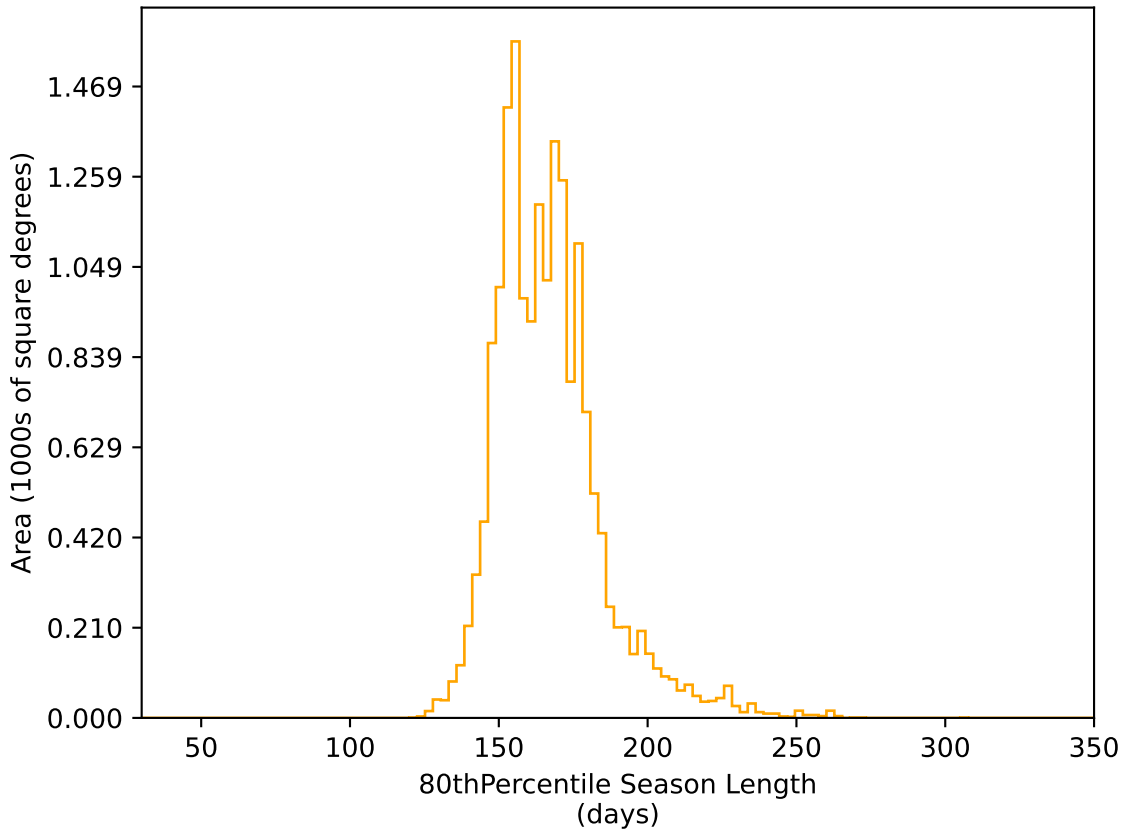
ddf_half_v3.4_10yrs WFD r band: 80thPercentile Season Length
