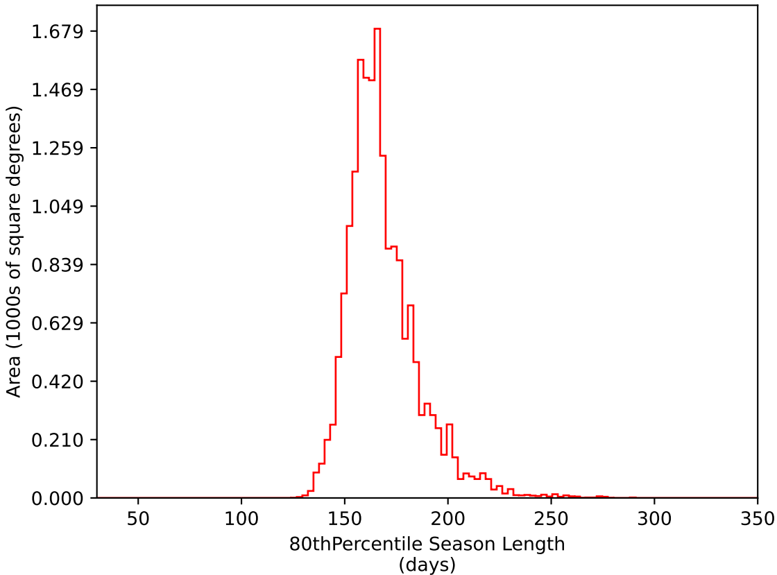
ddf_half_v3.4_10yrs WFD i band: 80thPercentile Season Length
