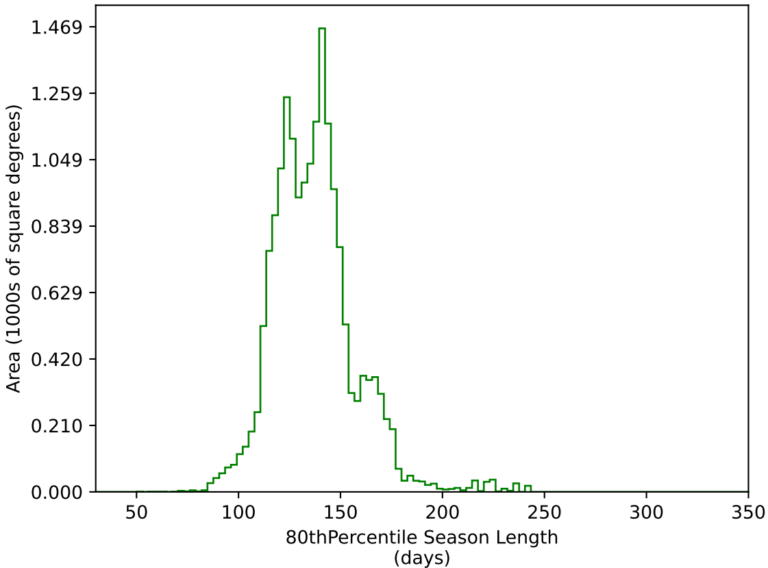
ddf_half_v3.4_10yrs WFD g band: 80thPercentile Season Length
