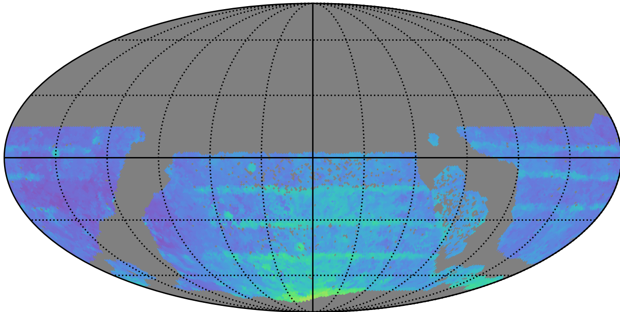
ddf_half_v3.4_10yrs WFD all bands: 80thPercentile Season Length
