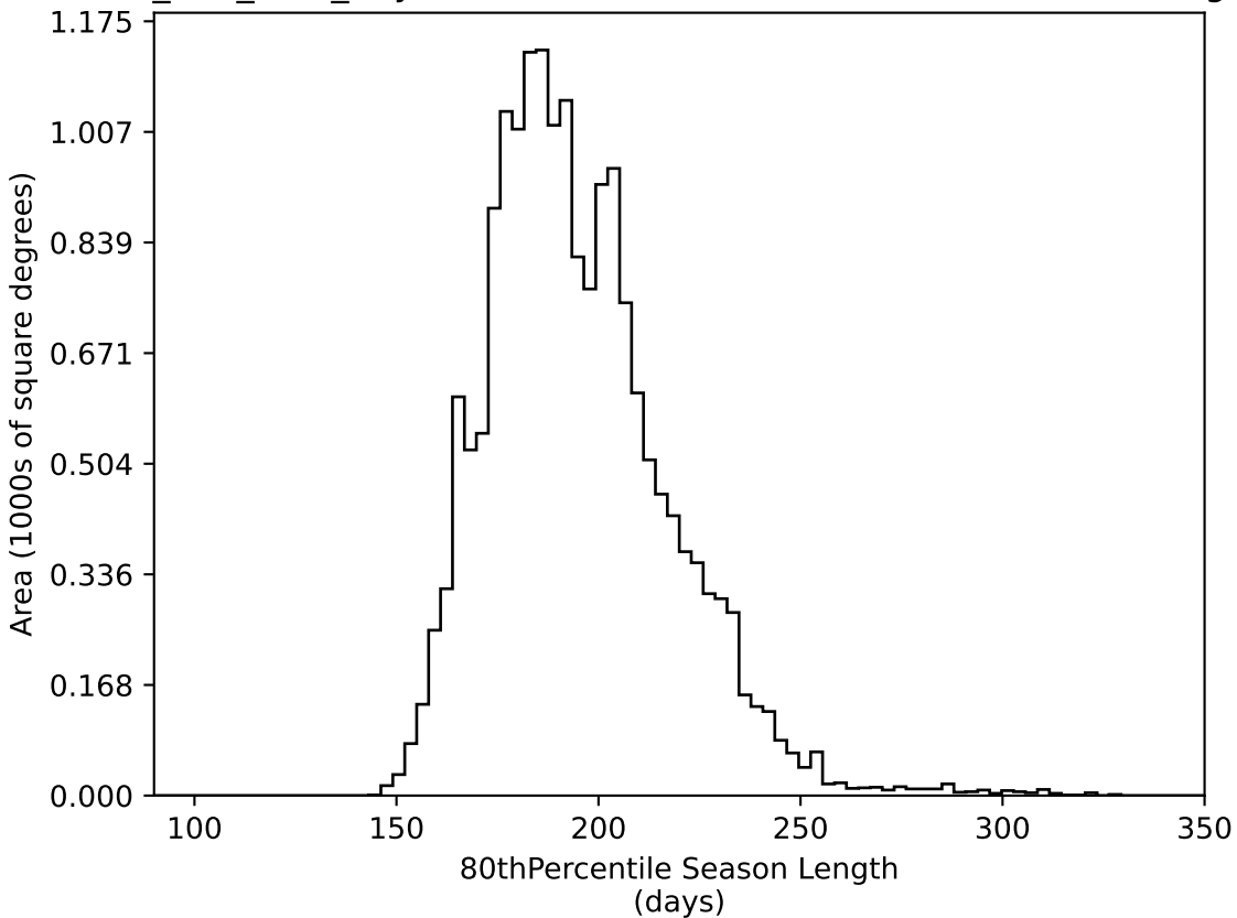
ddf_half_v3.4_10yrs WFD all bands: 80thPercentile Season Length
