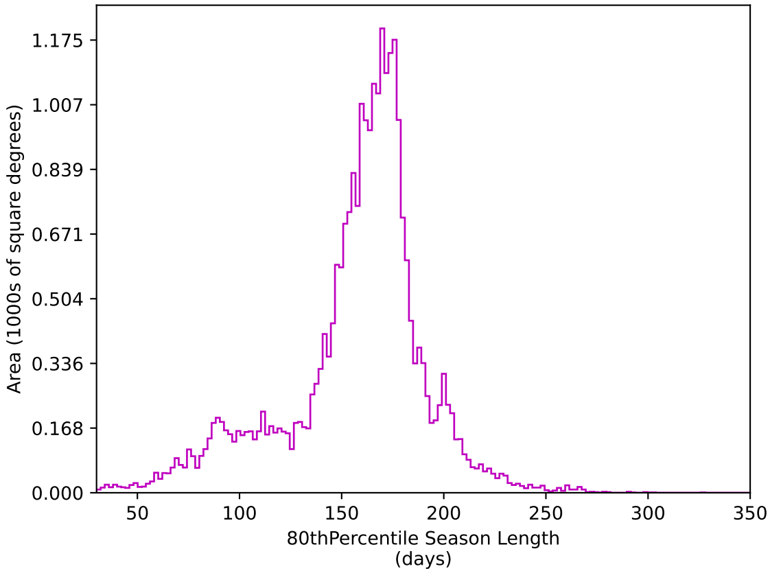
ddf_half_v3.4_10yrs All sky z band: 80thPercentile Season Length
