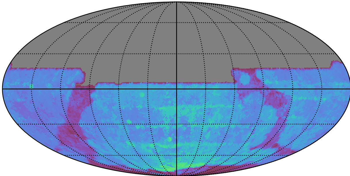
ddf_half_v3.4_10yrs All sky y band: 80thPercentile Season Length
