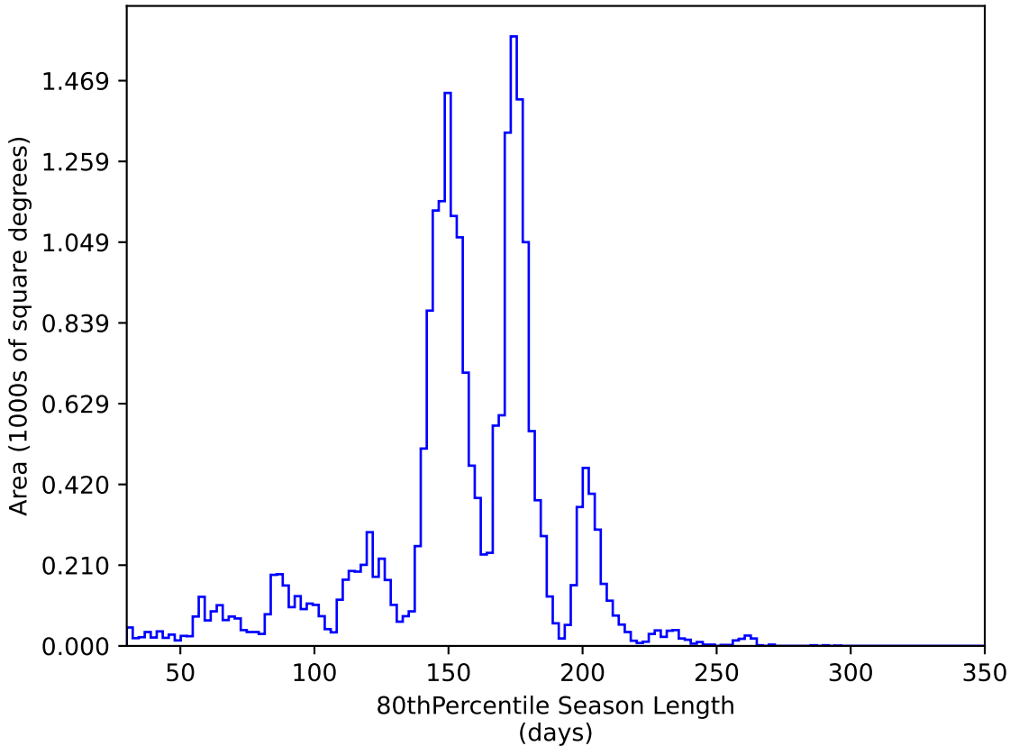
ddf_half_v3.4_10yrs All sky y band: 80thPercentile Season Length
