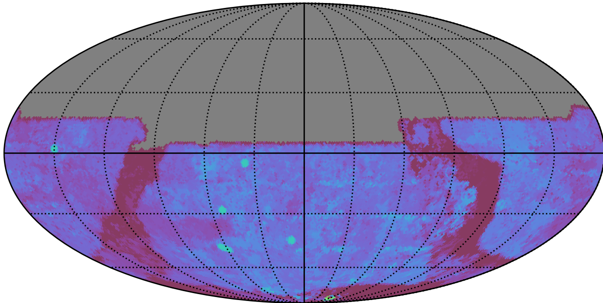
ddf_half_v3.4_10yrs All sky u band: 80thPercentile Season Length
